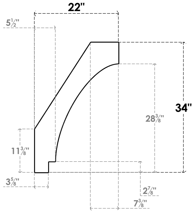
SIDE PROFILE
